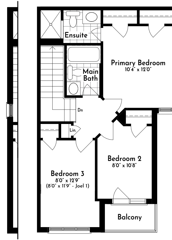
End. Cond. Joel 2 Upper Level
